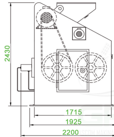
FLAKING ROLLER MILL GKV-RM-600
