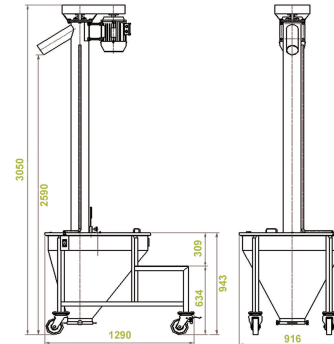
Screw Conveyor Vertical GDP-DH300
